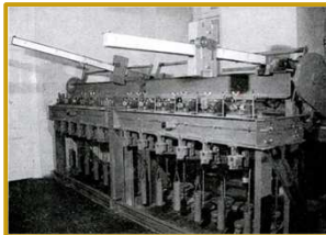
equipment developed by A. Casagrande and K. Terzaghi at TU Wien
